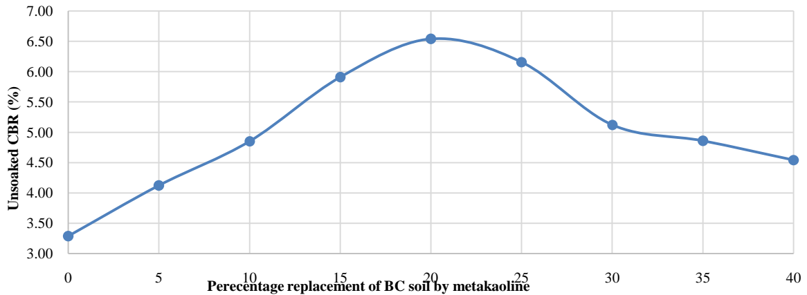
Figure 10 Variation of unsoaked CBR for different percentage replacement of BC soil by metakaoline
