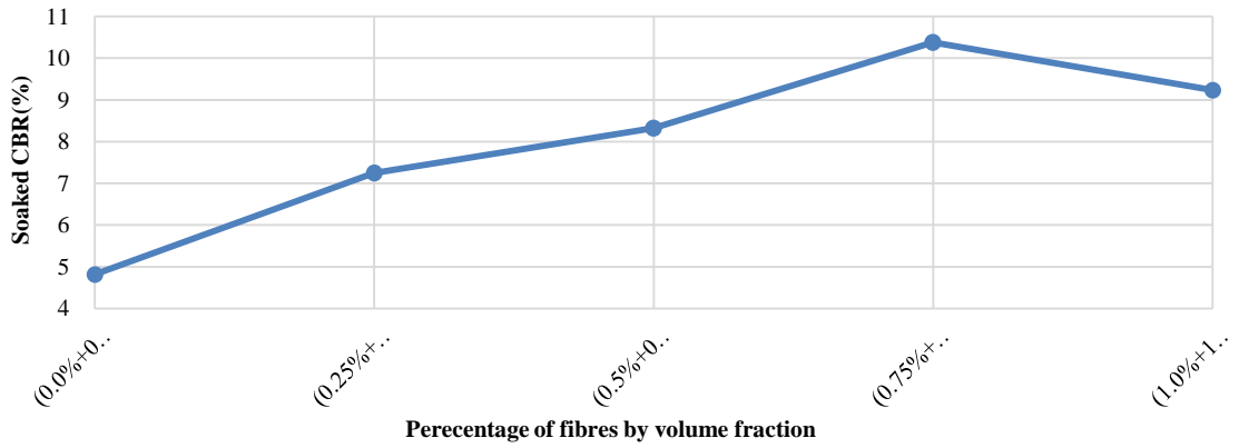
Figure 25 Variation of soaked CBR for different percentage of (PPF + HDPEF) when BC soil is replaced by metakaoline
