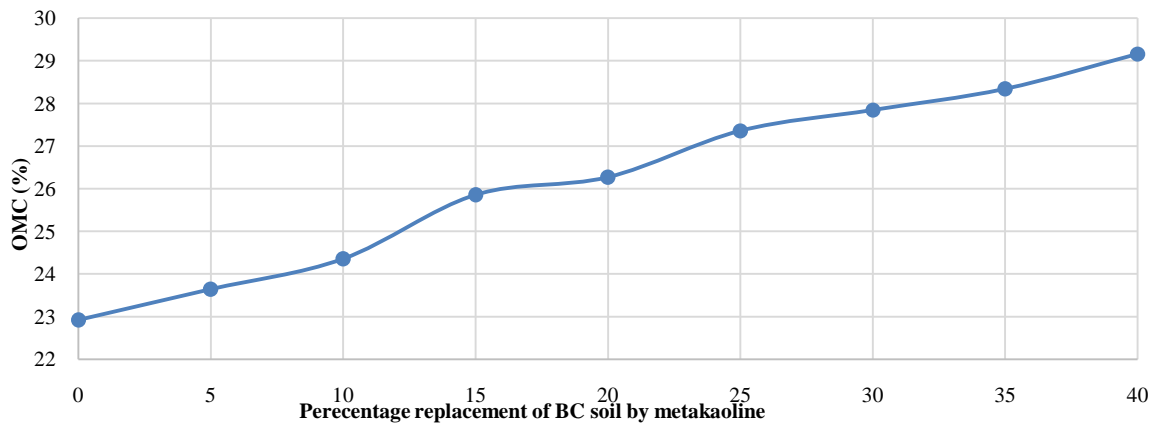
Figure 9 Variation of optimum moisture content for different percentage replacement of BC soil by metakaoline
