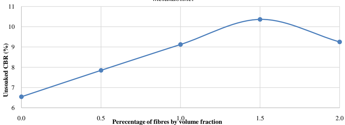
Figure 18 Variation of unsoaked CBR for different percentage of polypropylene fibres when BC soil is replaced by metakaoline.
