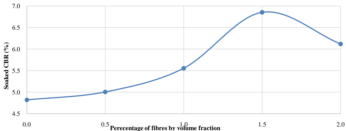
Figure 23 Variation of soaked CBR for different percentage of jute fibres when BC soil is replaced by metakaoline.
