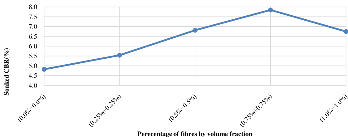
Figure 29 Variation of soaked CBR for different percentage of (JF + WPF) when BC soil is replaced by metkaoline
