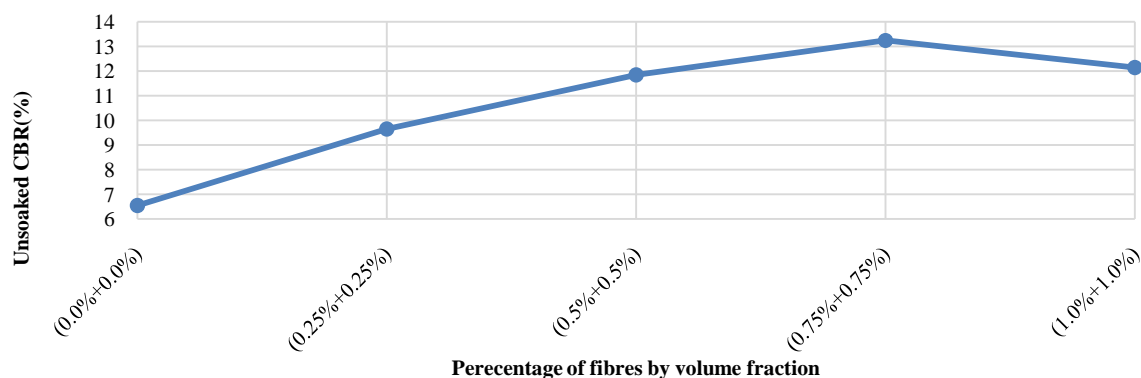
Figure 24 Variation of unsoaked CBR for different percentage of (PPF + HDPEF) when BC soil is replaced by metakaoline
