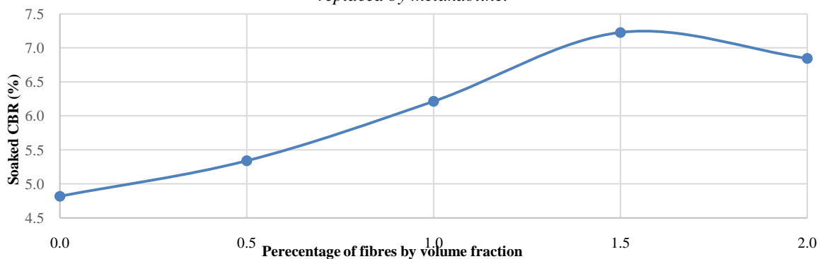
Figure 21 Variation of soaked CBR for different percentage of waste plastic fibres when BC soil is replaced by metakaoline.
