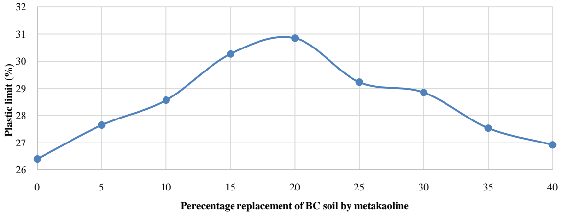
Figure 3 Variation of plastic limit for different percentage replacement of BC soil by metakaoline
