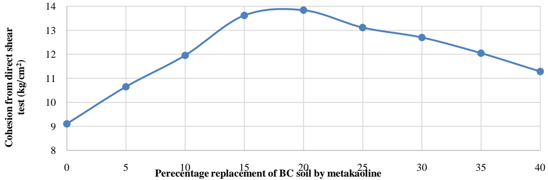
Figure 12 Variation of cohesion of direct shear test for different percentage replacement of BC soil by metakaoline
