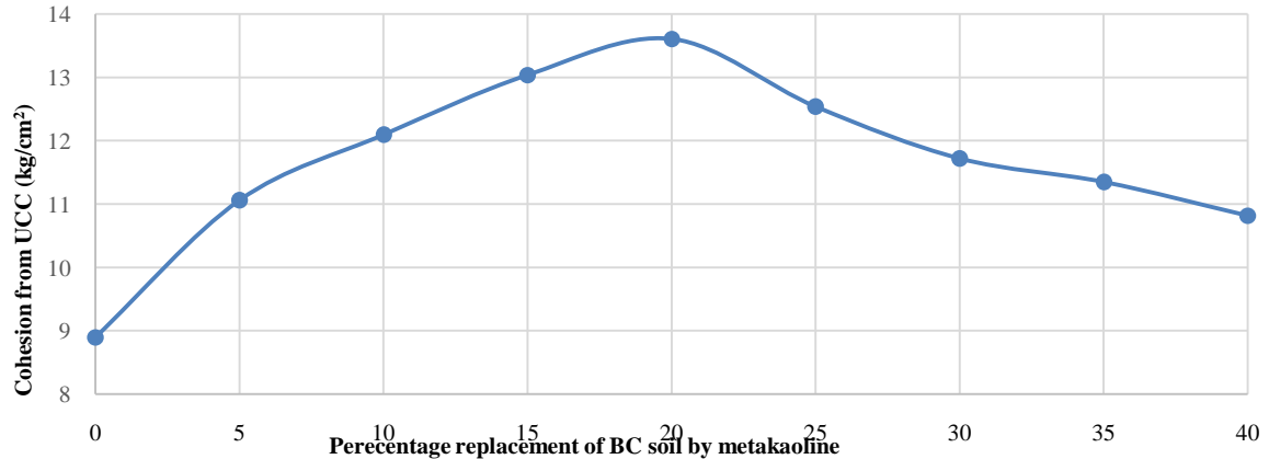
Figure 14 Variation of Cohesion of UCC test for different percentage replacement of BC soil by metakaoline
