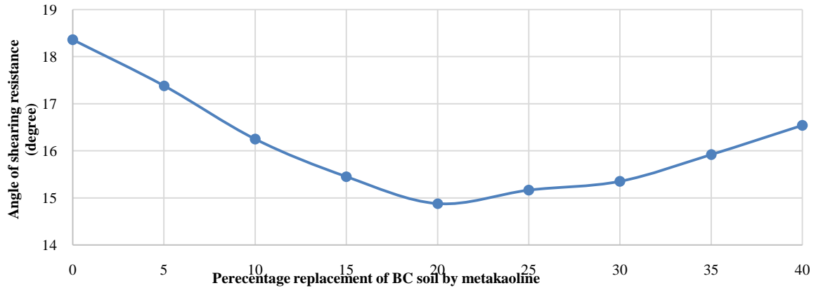
Figure 13 Variation of angle of shearing resistance of direct shear test for different percentage replacement of BC soil by metakaoline
