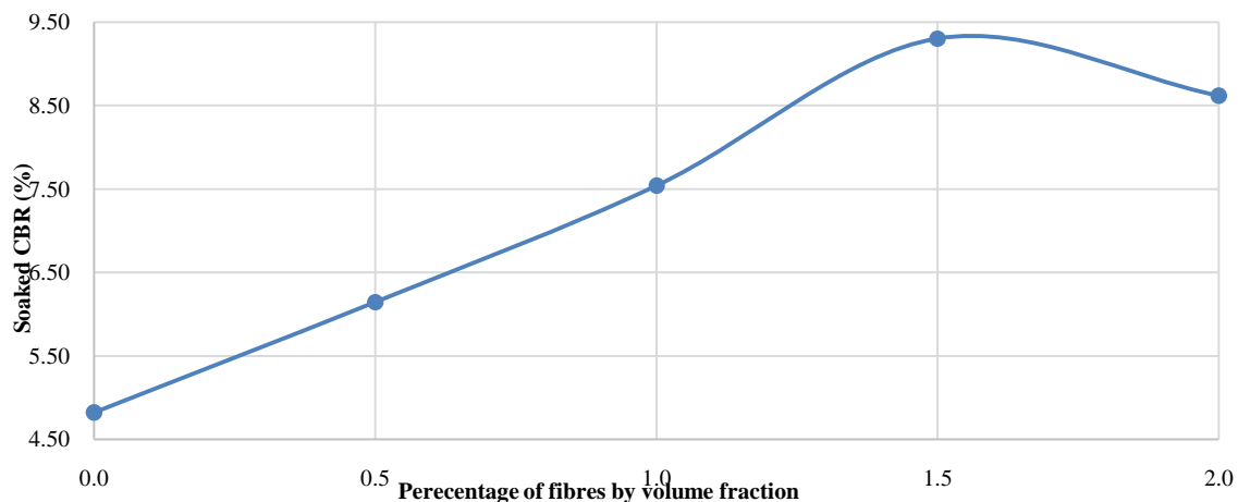
Figure 17 Variation of soaked CBR for different percentage of HDPE fibres when BC soil is replaced by metakaoline.
