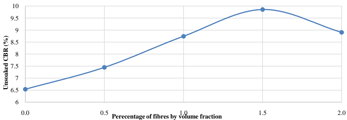
Figure 20 Variation of unsoaked CBR for different percentage of waste plastic fibres when BC soil is replaced by metakaoline.
