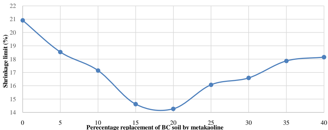
Figure 6 Variation of shrinkage limit for different percentage replacement of BC soil by metakaoline
