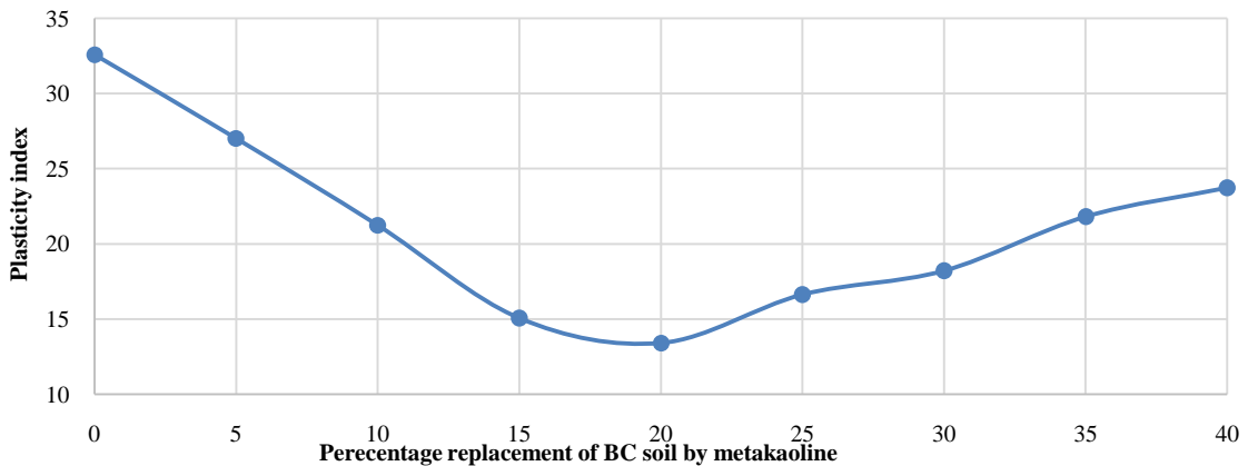
Figure 5 Variation of plasticity index for different percentage replacement of BC soil by metakaoline
