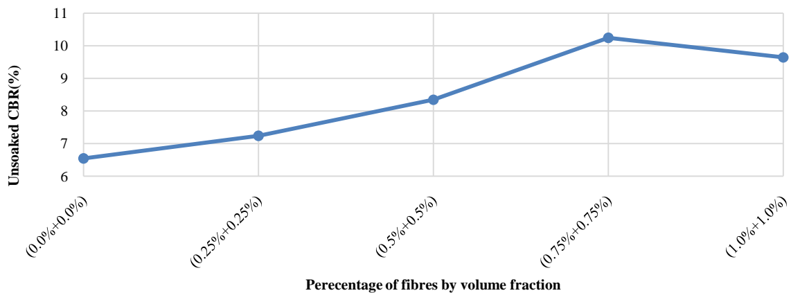
Figure 28 Variation of unsoaked CBR for different percentage of (JF + WPF) when BC soil is replaced by metakaoline
