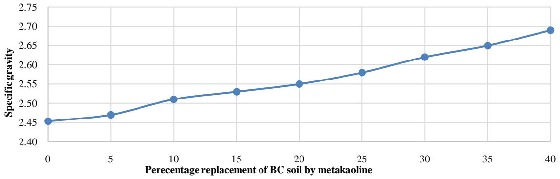
Figure 2 Variation of specific gravity for different percentage replacement of BC soil by metakaoline
