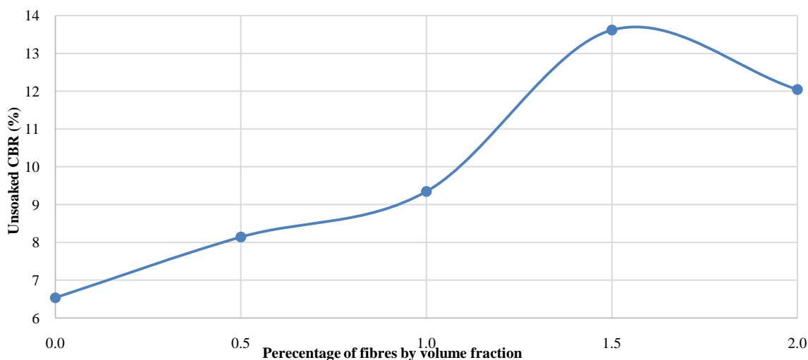
Figure 16 Variation of unsoaked CBR for different percentage of HDPE fibres when BC soil is replaced by metakaoline.
