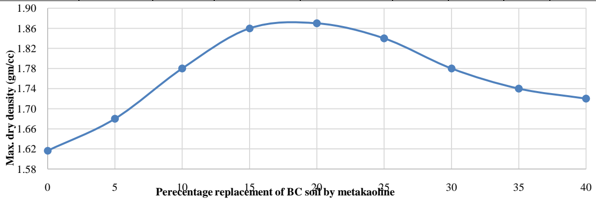
Figure 8 Variation of max. dry density for different percentage replacement of BC soil by metakaoline
