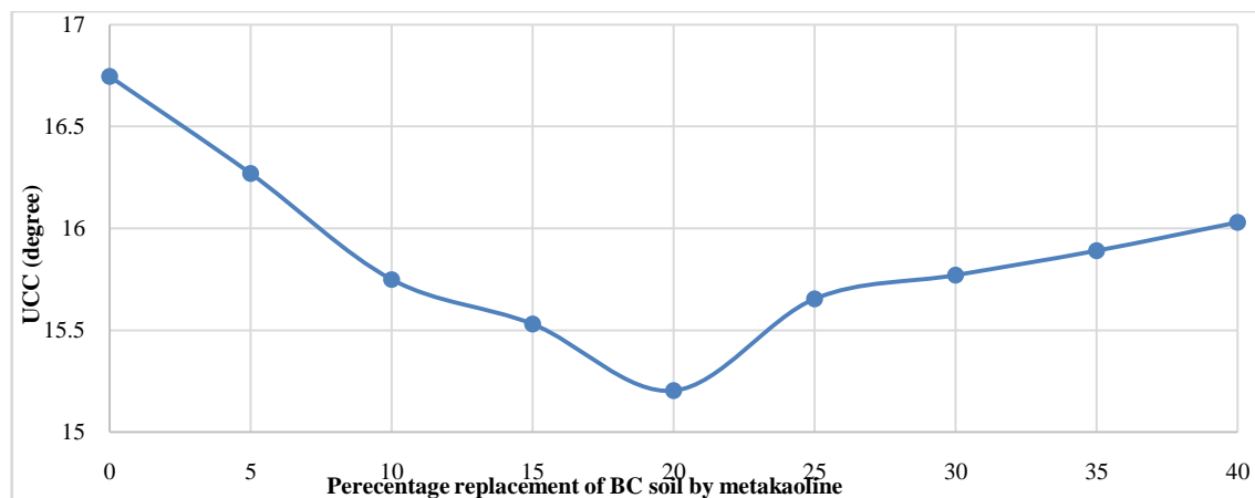
Figure 15 Variation of \alpha of UCC test for different percentage replacement of BC soil by metakaoline
