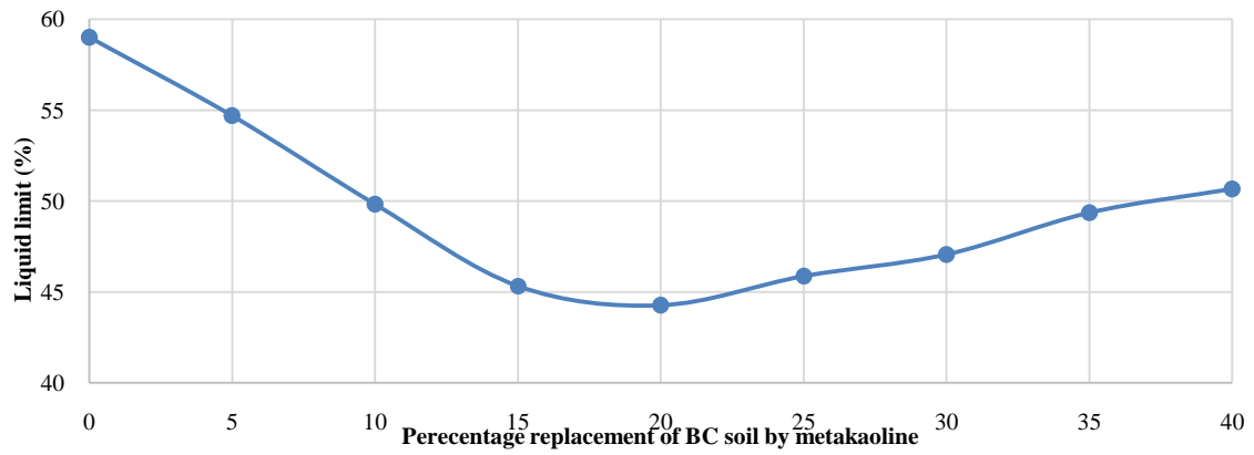
Figure 4 Variation of liquid limit for different percentage replacement of BC soil by metakaoline
