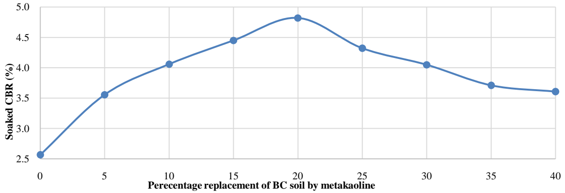
Figure 11 Variation of soaked CBR for different percentage replacement of BC soil by metakaoline
