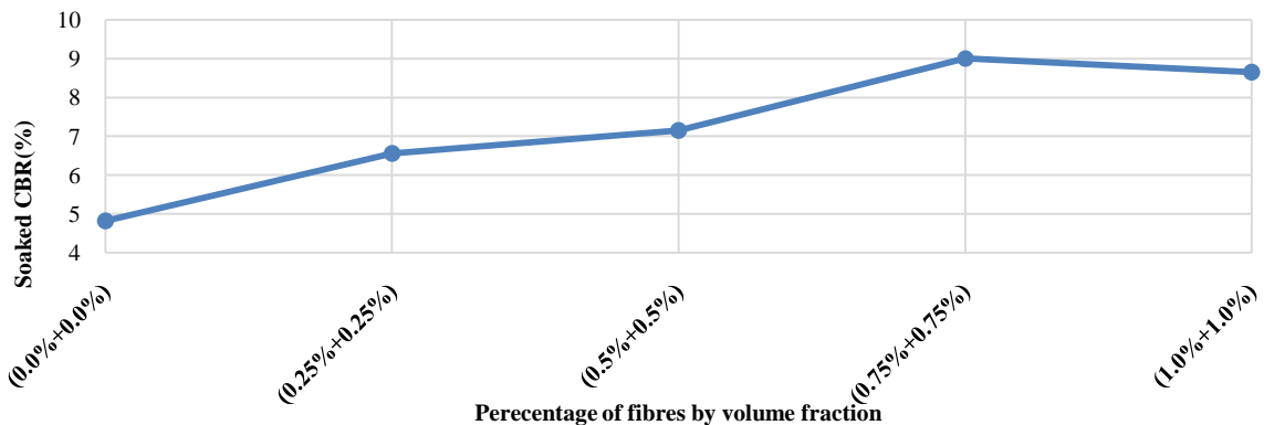
Figure 27 Variation of soaked CBR for different percentage of (PPF + WPF) when BC soil is replaced by metakaoline
