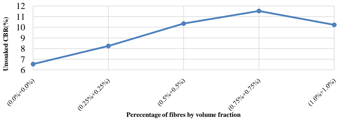
Figure 26 Variation of unsoaked CBR for different percentage of (PPF + WPF) when BC soil is replaced by metakaoline
