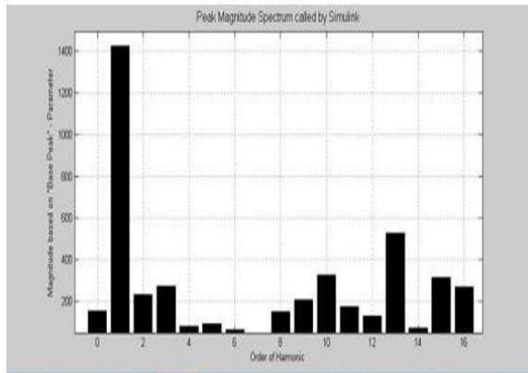
Fig 13. PV Harmonic output before filter.
