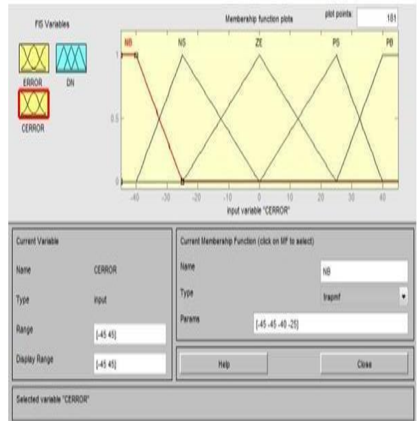
Fig 9. MF of the change in Error designed rule-based rule. Membership function of output designed to the rule-based rule is shown below.
