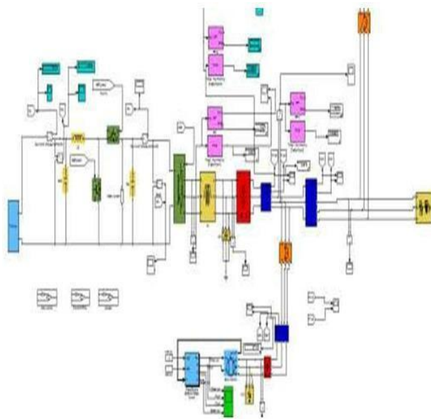
Fig 11. Simulation model.
