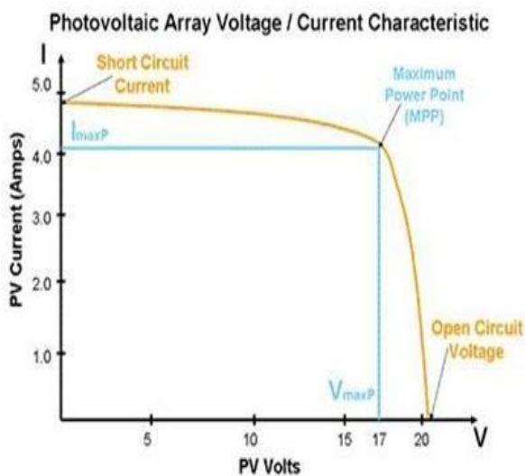
Fig 3. V-I characteristic.
