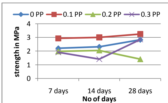
Fig.5. Compressive Strength Variation with No of Days
