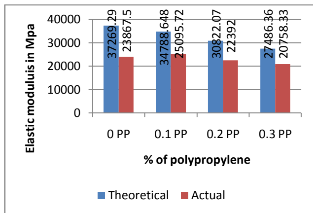
Fig6. Variations of elastic modulus with % of polypropylene.
