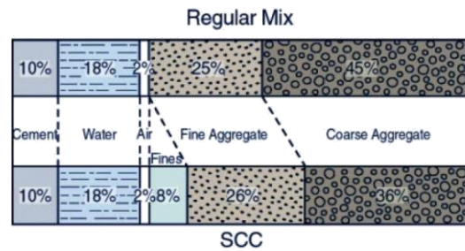
Fig. 1. Regular Mix Vs SCC
