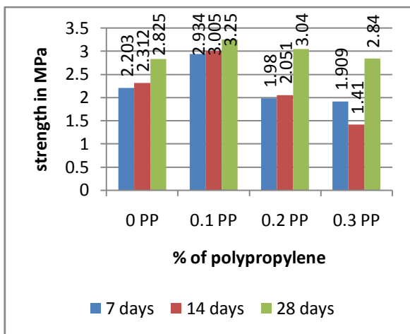
Fig.4. Split tensile Strength Variation with % of Polypropylene.
