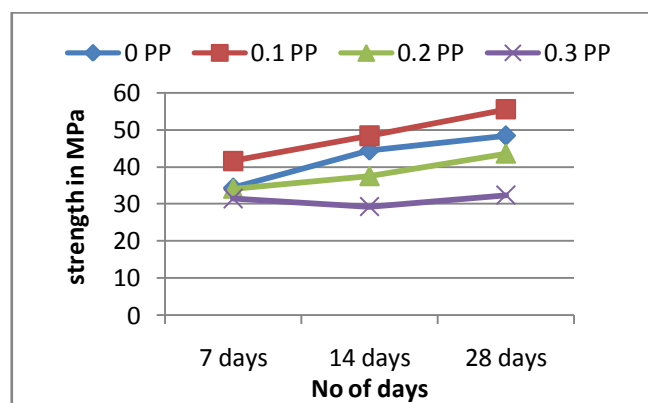
Fig.3. Compressive Strength Variation with No of Days
