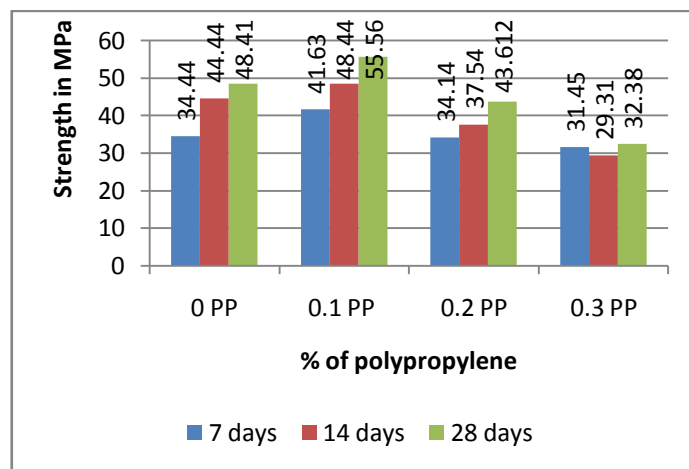
Fig.2. Compressive Strength Variation with % of Polypropylene
